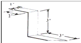
SAFING CLIP
