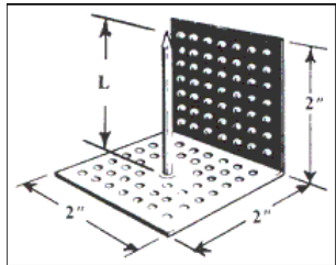
90° INSULATION HANGER
